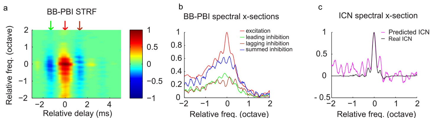
Fig 7. Constructive and destructive interference through integration of broadband PBI explains frequency sharpening of ICNs. (a) Population-average broadband PBI STRF has leading (green arrow) and lagging (brown arrow) inhibition around a central broadband excitatory domain (red arrow). (b) The spectral cross-sections are shown for the excitatory domain (red) along with the leading (green) and lagging (brown) inhibition and the summed inhibition (blue, leading + lagging component). The excitation has a sharp central peak around 0 octave frequency and adjacent peaks at intervals of approximately 0.28 octave. The summed inhibition has a broad profile with peaks that are spectrally displaced (out of phase) with the excitatory peaks. Upon summing the excitation and inhibition, the broad spectral structure cancels, and the narrowly tuned central region is preserved (panel c, magenta), which predicts the sharpened frequency tuning observed for ICNs (panel c, black, population-average ICN spectral cross-section). Underlying data can be found in S7 Data and S7 Code . BB, broadband; ICN, inferior colliculus neuron; PBI, putative brainstem input; STRF, spectrotemporal receptive field.
