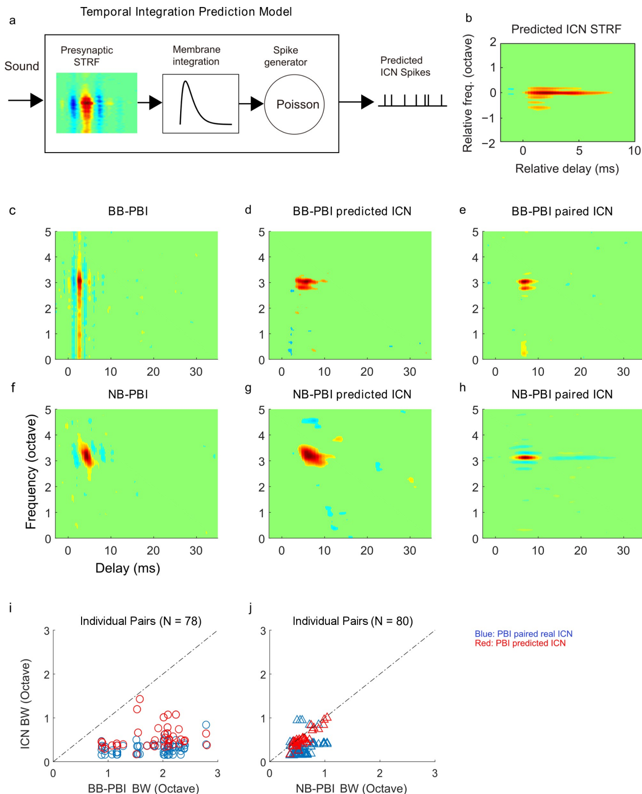
Fig 8. Temporal integration mechanism for sharpening frequency selectivity in ICNs. (a) A neuron model was developed to test the hypothesis that frequency selectivity can be sharpened through temporal integration of the converging broadband PBI. The model includes the PBI receptive field to account for presynaptic integration, a cell membrane integration compartment, and a Poisson spike train generator. When applied to the average broadband PBI STRF, the resulting STRF from the model spike train output sharpens dramatically and has similar spectral tuning and temporal profile
