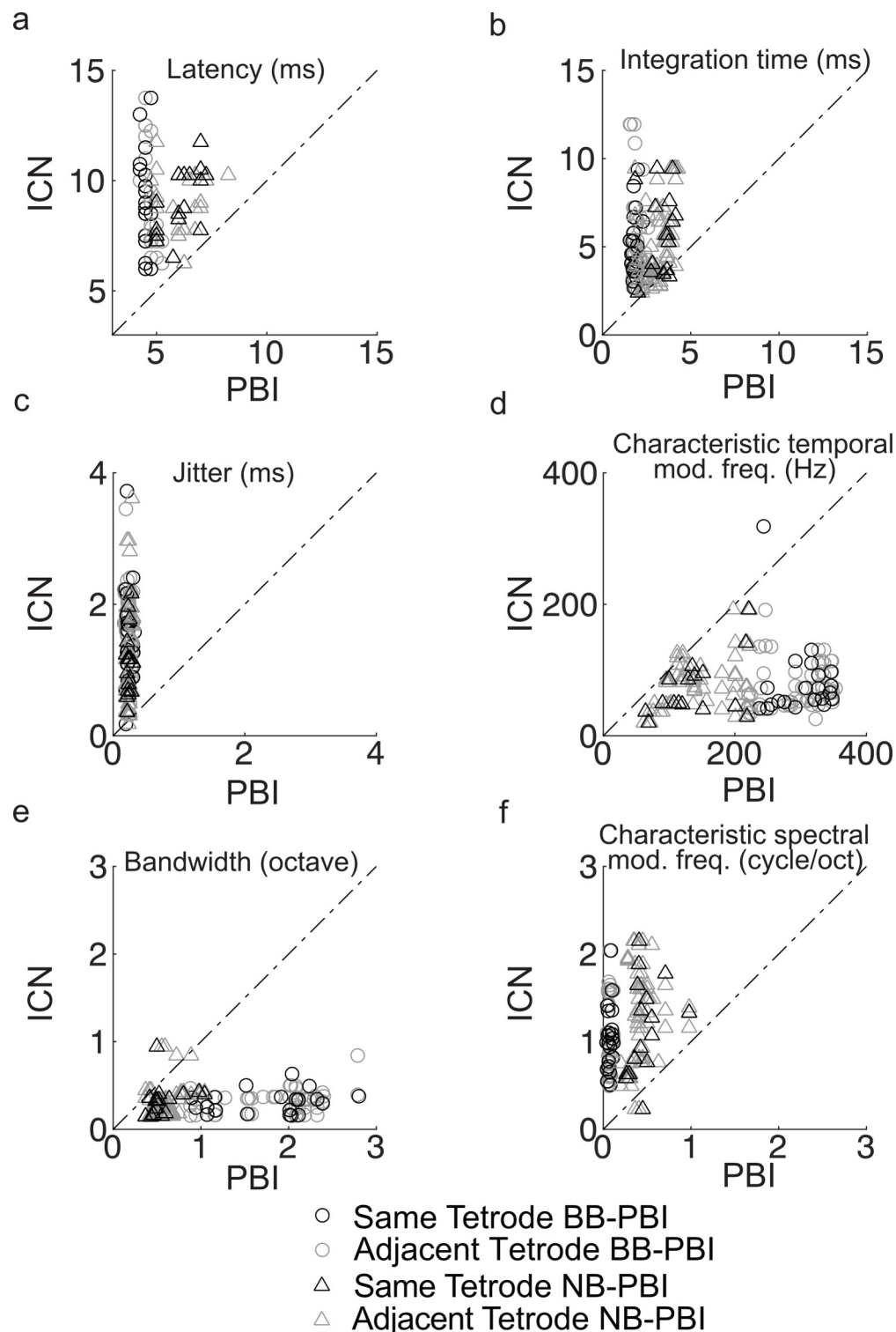
Fig 5. Temporal resolution degrades and spectral resolution is enhanced for ICNs. PBIs exhibit shorter response latency (panel a, 4.9 versus 8.6 ms), shorter integration time (panel b, 2.3 versus 4.3 ms), substantially higher spike-timing precision (panel c, jitter = 0.2 versus 1.2 ms), and better temporal modulation sensitivity (panel d, 222 versus 72 Hz) when compared to their paired ICNs. In contrast, ICNs have substantially narrower bandwidth than PBIs (panel e, 0.33 versus 0.94 octave) and prefer finer spectral modulations (panel f, 1.1 versus 0.2 cycle/octave). Open circle denotes broadband PBI, and triangle denotes narrowband PBI. Pairs recorded from the same tetrode are shown in black, and
