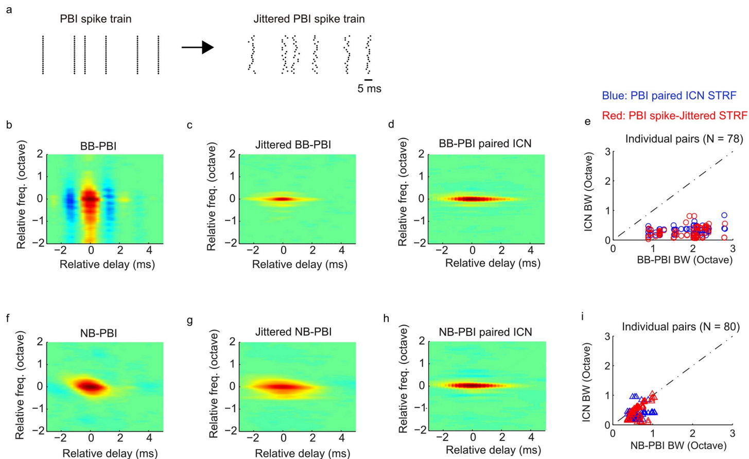
Fig 6. Reduced spike-timing precision enhances frequency selectivity of broadband PBIs but not for narrowband PBIs. (a) Synthetic spike-timing jitter (1.5 ms) was added to each of the PBI spike trains, and the STRF was recomputed. Although the population-average broadband PBI is broadly tuned (b), the jittered broadband PBI is substantially narrower (c) and closely matches the population-average ICN STRF at those sites (d). This enhanced frequency selectivity was evident after adding spike-timing jitter for each of the individual broadband PBIs (panel e, red dots: broadband PBI versus jittered broadband PBI bandwidth) and closely matched the observed measurements for individual paired broadband PBIs and ICNs (panel e, blue dots: broadband PBI versus ICN bandwidth). This behavior was not evident for narrowband PBIs (f–i) because the population-average STRF bandwidth was similar before (f) and after (g) adding spike-timing jitter. Furthermore, bandwidths before and after adding spike-timing jitter for individual narrowband PBIs (i) were significantly correlated ( r = 0.6 \pm 0.12 ), implying that the bandwidth after adding spike-timing jitter was largely inherited from the original narrowband PBI. Underlying data can be found in S6 Data and S6 Code . BB, broadband; ICN, inferior colliculus neuron; NB, narrowband; PBI, putative brainstem input; STRF, spectrotemporal receptive field.
