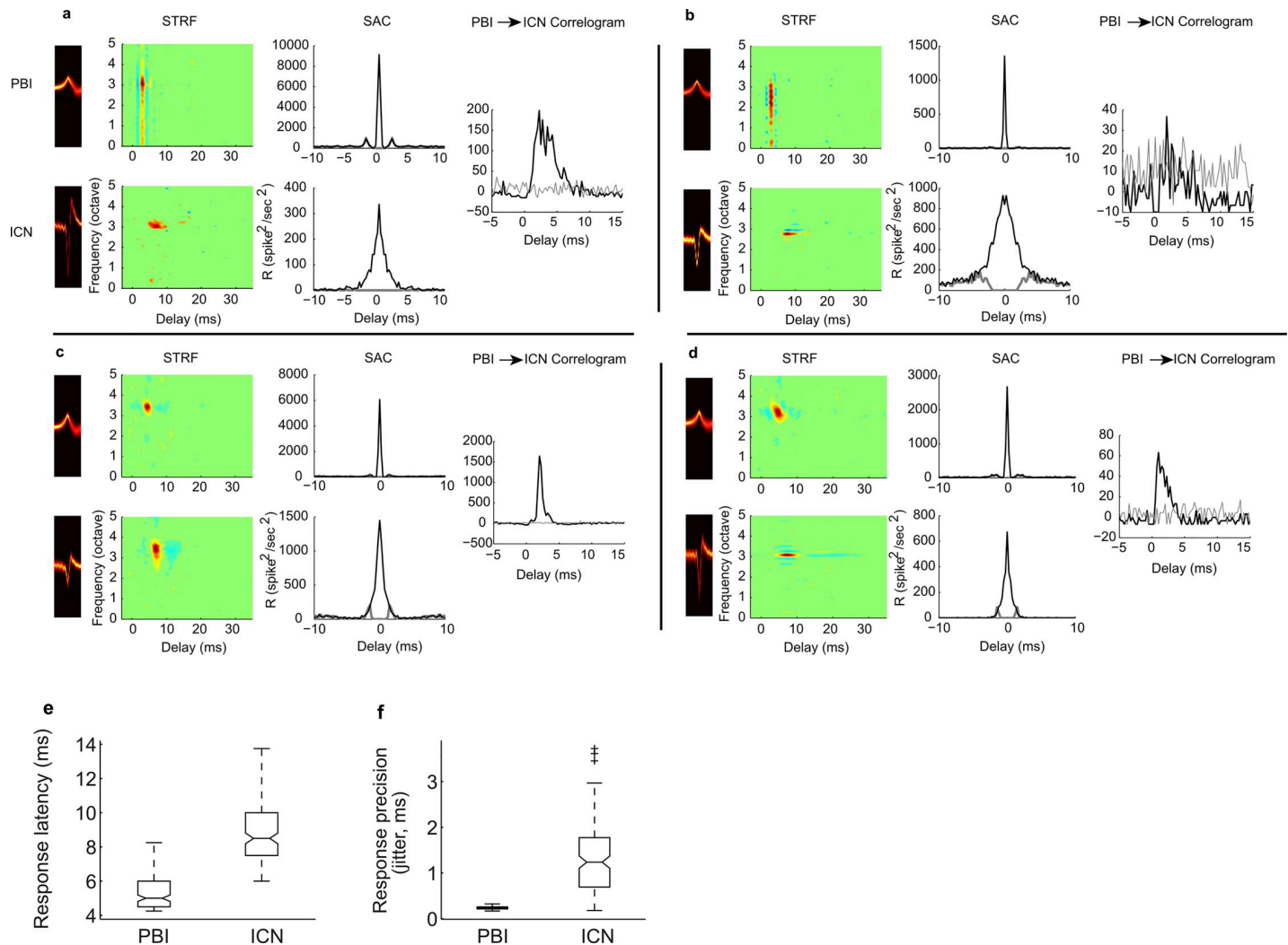
Fig 2. Spiking and spectrotemporal integration characteristics of PBI-ICN pairs recorded from the same tetrode. In each example, we show the STRFs (left panels, top row for PBI and bottom row for ICN), the spike train SACs (middle panels), and the crosscorrelation between PBI and ICN (right panel). Only statistically significant samples of the STRF ( p < 0.001 ) are shown, and samples that do not exceed the significance threshold are set to zero (same convention for all figures; red indicates excitatory response above the baseline firing rate, blue indicates suppressive and/or inhibitory response, and green is the baseline activity). The units of frequency are in octave relative to 1 kHz. As seen in these 4 examples, PBIs often have broader bandwidths than ICNs (panels a, b, d). PBIs also exhibit shorter response latency and faster integration times (panels a–d). Finally, spike-timing precision is higher for PBIs as seen in the SAC (panels a–d, gray line corresponds to the unshuffled autocorrelogram with central peak removed). Significant correlated activity was observed in the PBI-ICN crosscorrelation between 0 to 5 ms delay in 89% of PBI-ICN pairs ( t test, p < 0.001 , gray line corresponds to the interspike interval shuffled crosscorrelation). Overall, PBIs have shorter response latencies (panel e; range 4.2–8.2 ms; median 4.9 ms) and higher temporal precision (panel f; spike-timing jitter: range 0.17–0.32 ms; 0.23 ms median) compared to that of ICNs (latency range 6–13.8 ms; 8.5 ms median; jitter range 0.2–3.7 ms; 1.2 ms median, respectively). Underlying data can be found in S2 Data and S2 Code . ICN, inferior colliculus neuron; PBI, putative brainstem input; SAC, shuffled autocorrelogram; STRF, spectrotemporal receptive field.
